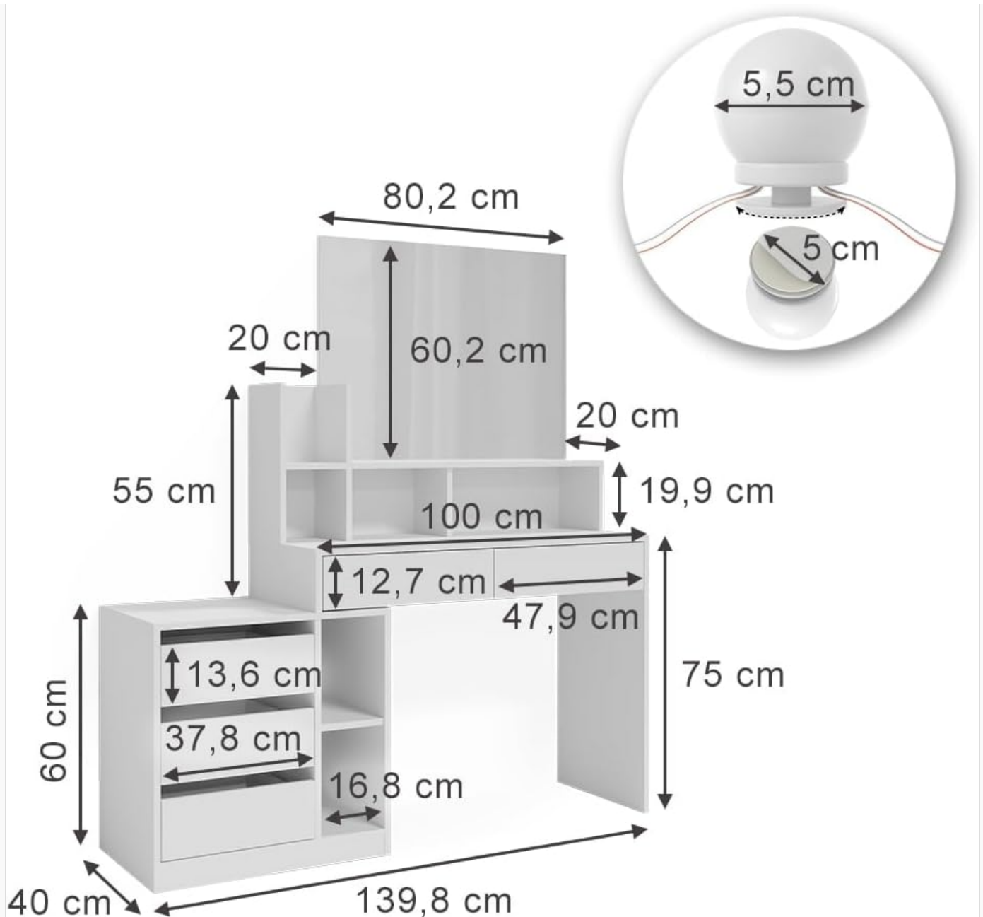
Figure 3.1: Product dimensions and LED bulb details. Overall dimensions: 139.8 cm (width) x 40 cm (depth) x 115 cm (height).
