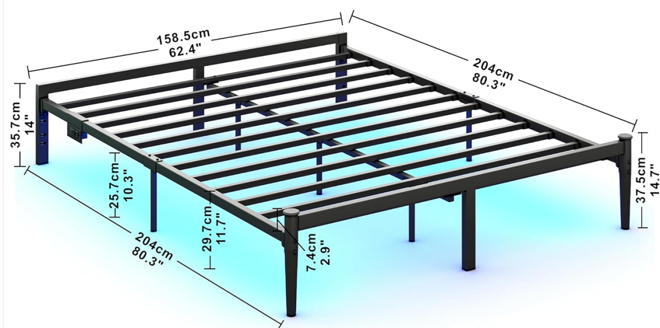
Image: A technical diagram illustrating the length, width, and height dimensions of the Queen Size LIKIMIO bed frame.
