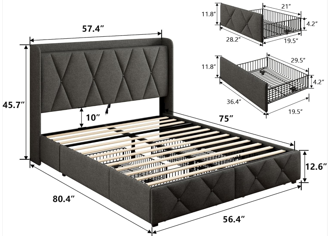
Figure 1: Product Dimensions and Drawer Sizes.
