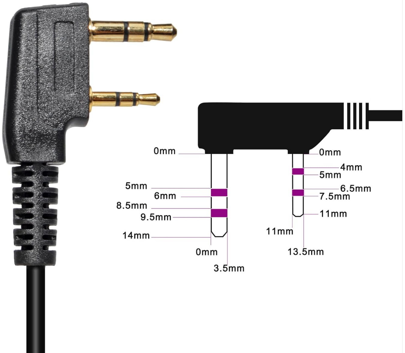
Image: A detailed diagram illustrating the universal 2-pin connector dimensions and configuration, compatible with Baofeng and Kenwood radios.
