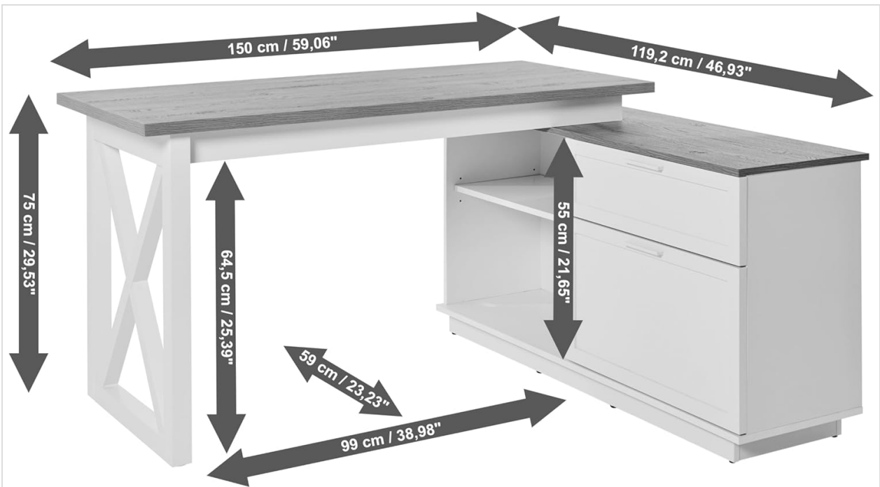
Figure 3: Detailed dimensions of the desk, including overall width (150 cm), depth (119.2 cm), and height (75 cm).
