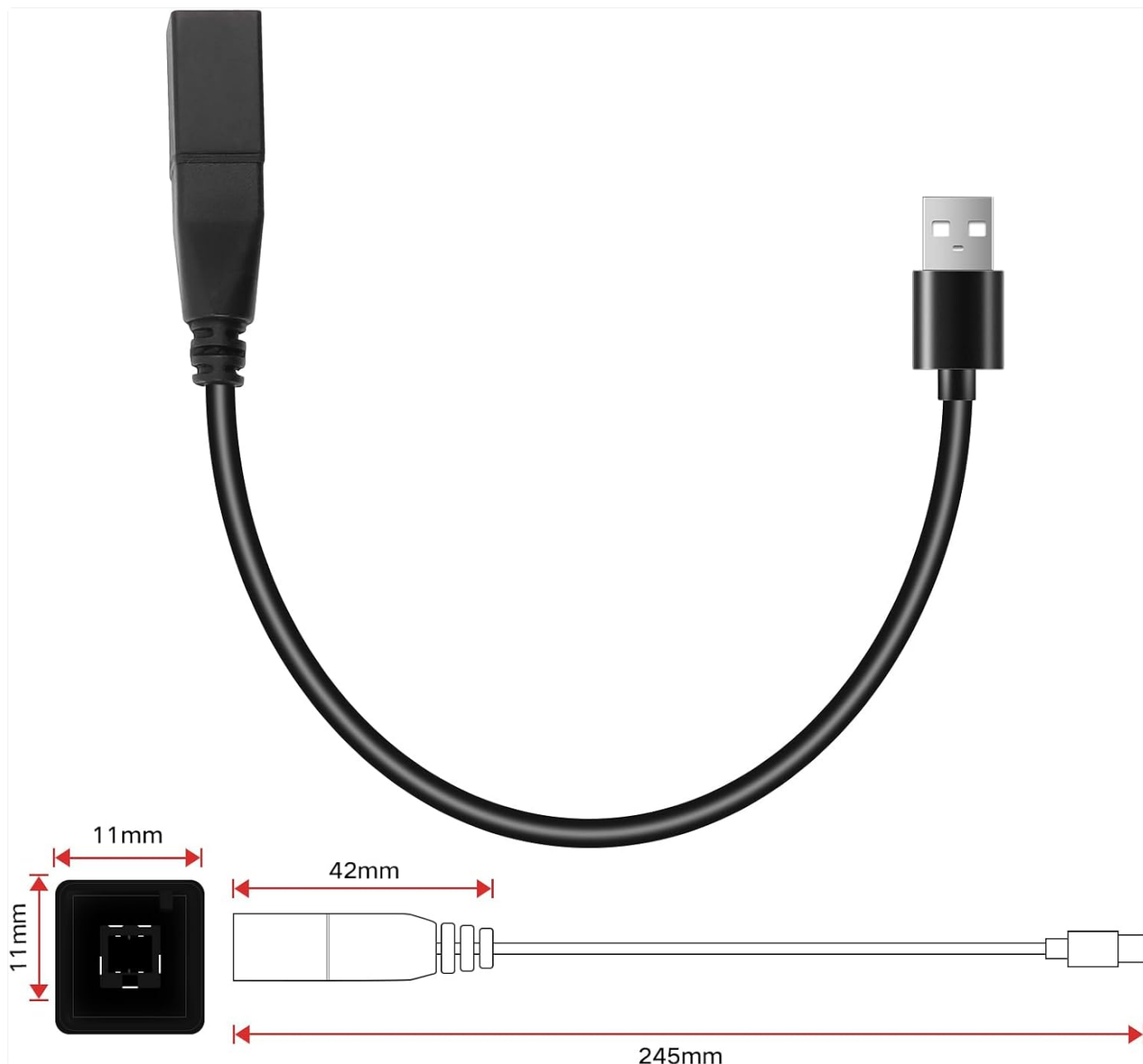
Image: Technical drawing showing the dimensions of the ViaBecs USB-FT03 adapter.
