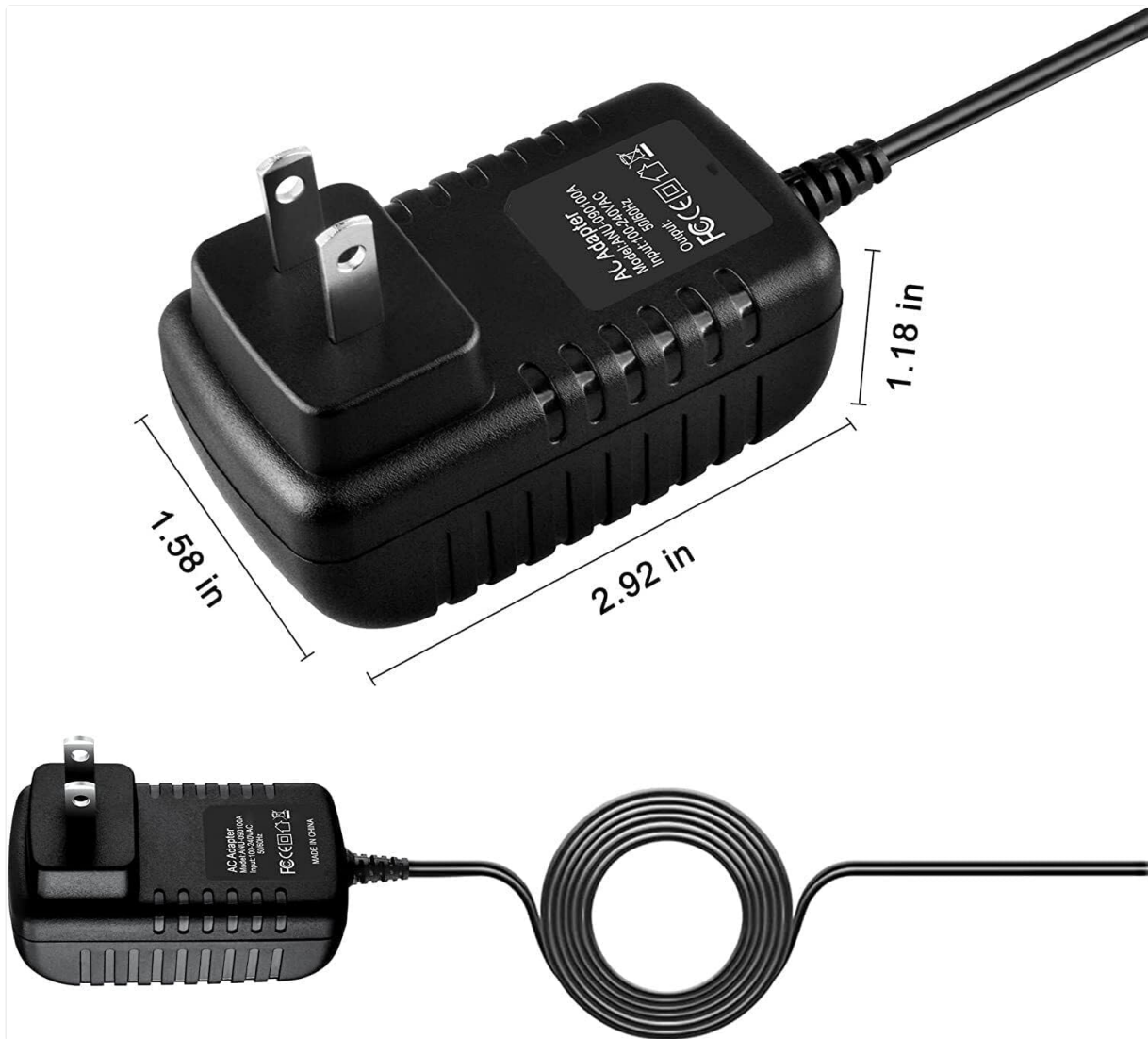
Image 4: Marg 9VDC 1A AC Adapter with indicated dimensions. This image illustrates the Marg 9VDC 1A AC Adapter with its physical dimensions labeled, showing its length, width, and height for size reference.
