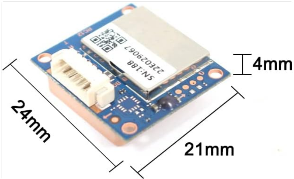
Figure 3.1: Dimensions of the YIWENG GPS Chip Module. The module measures approximately 24mm in length, 21mm in width, and 4mm in height.
