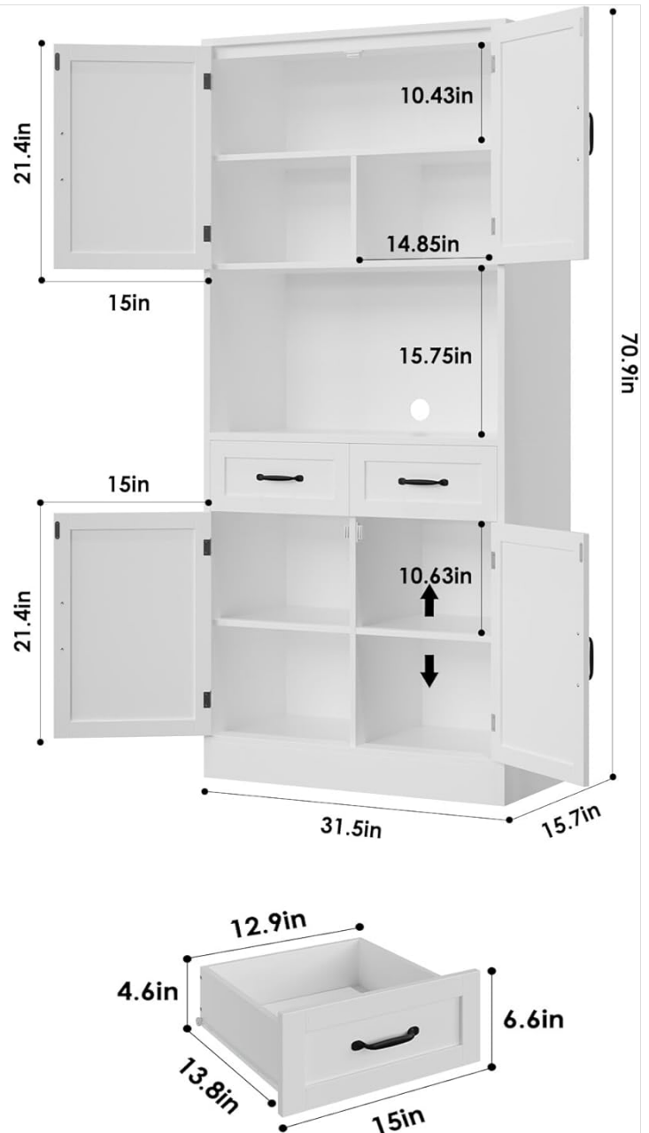
Figure 2.1: Cabinet Dimensions and Capacities
