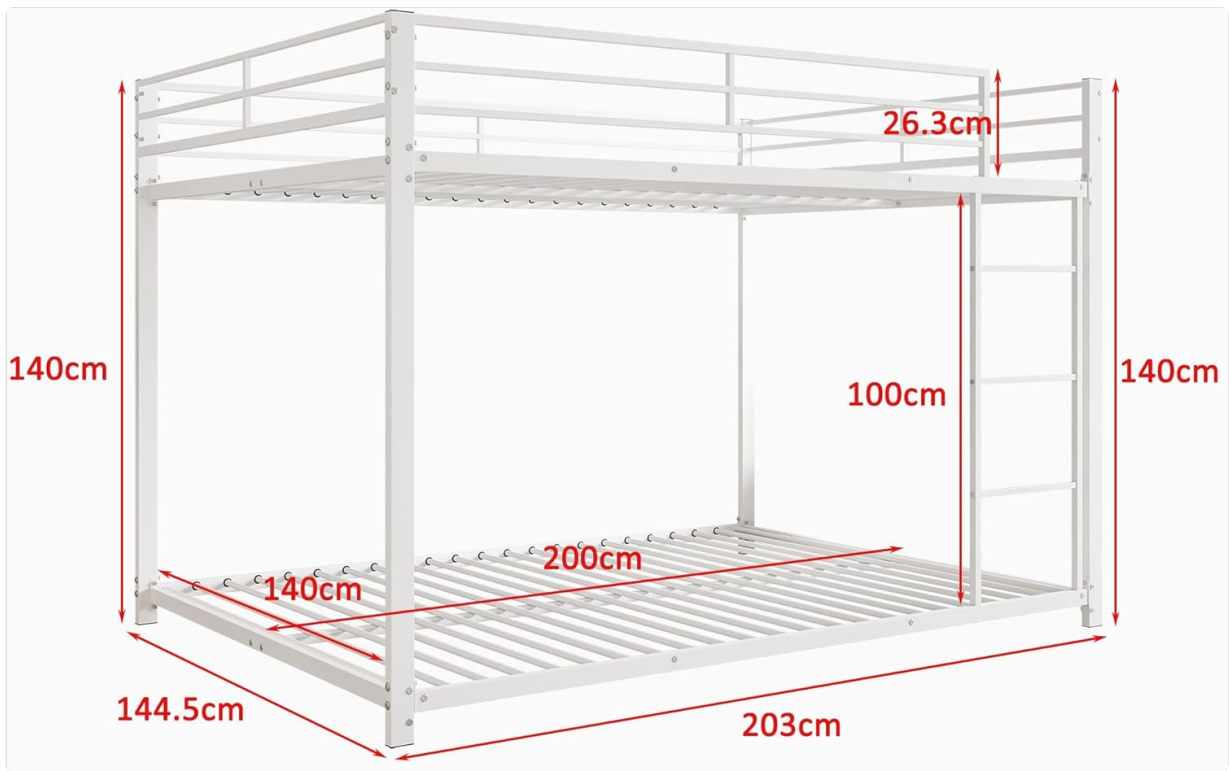
Figure 1: Dimensional diagram of the Moimhear Metal Bunk Bed (L: 203cm, W: 145cm, H: 140cm).
