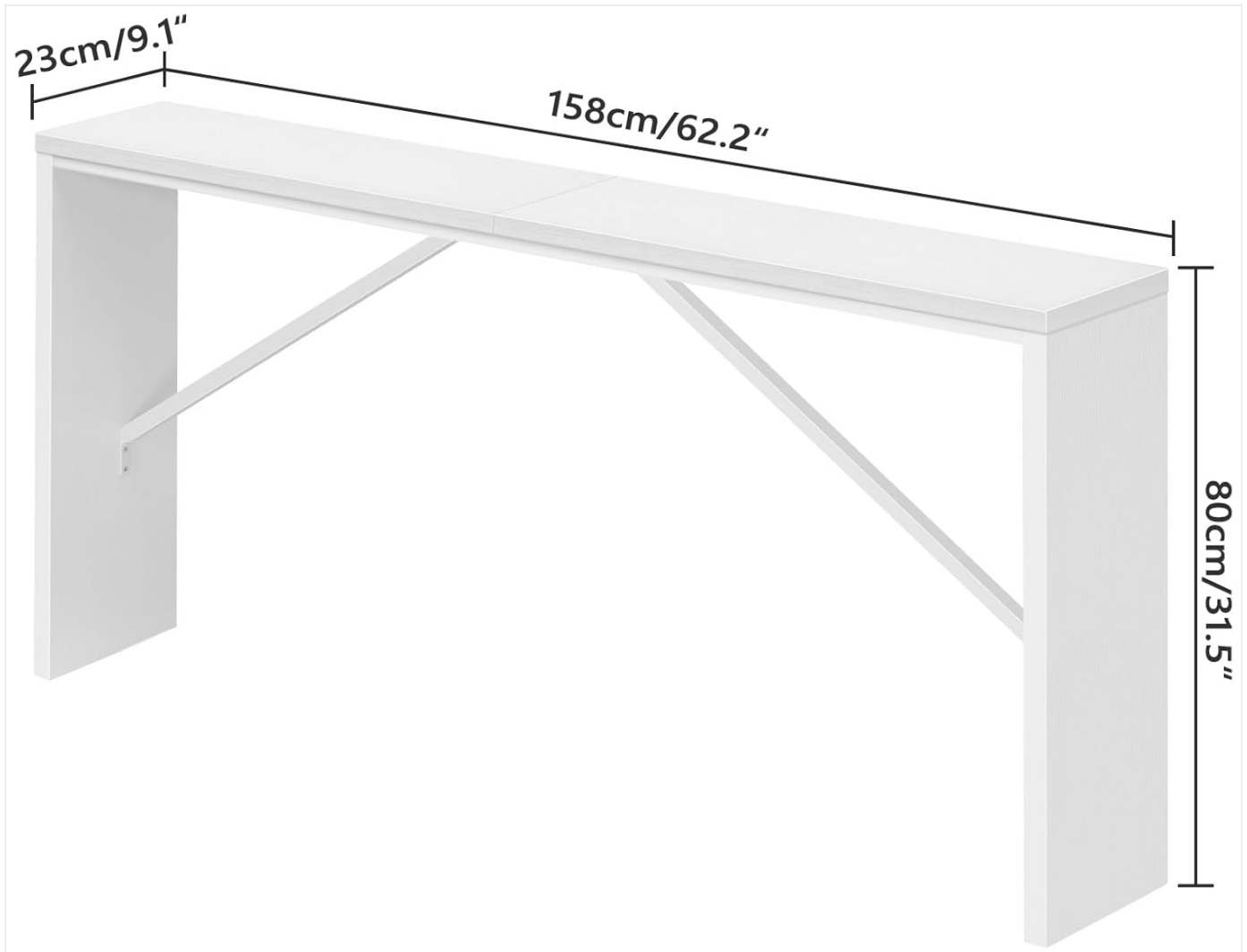
Figure 2: Product Dimensions
