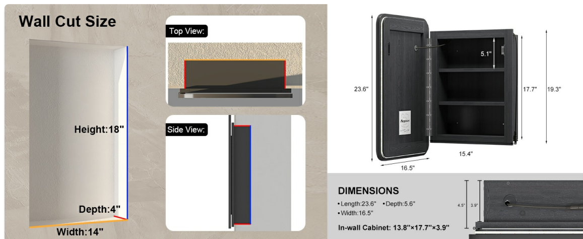
Image 5.2: Wall Cut Size and Dimensions
