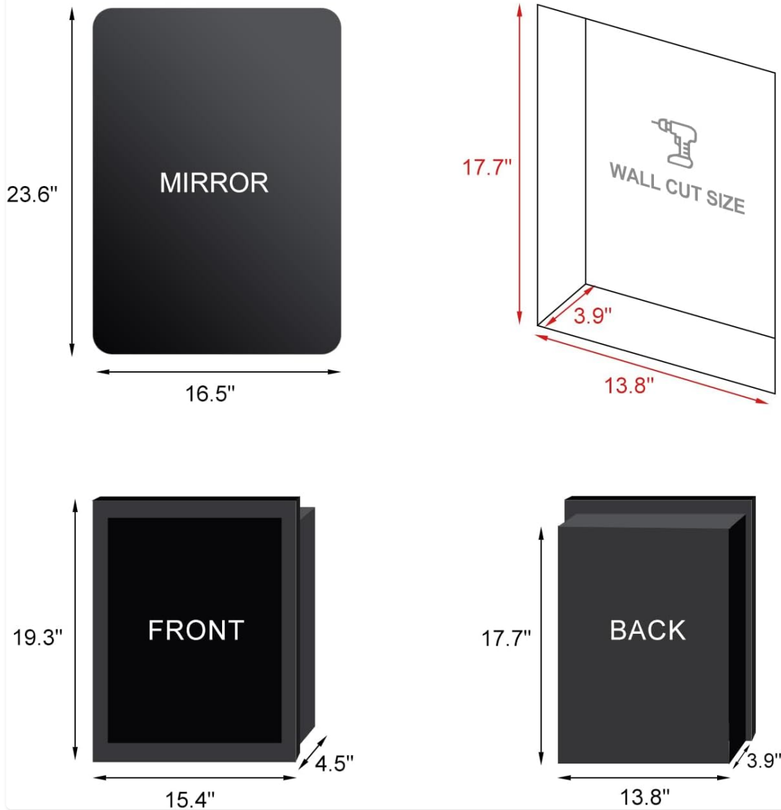
Image 5.1: Recessed Medicine Cabinet Size Diagram
