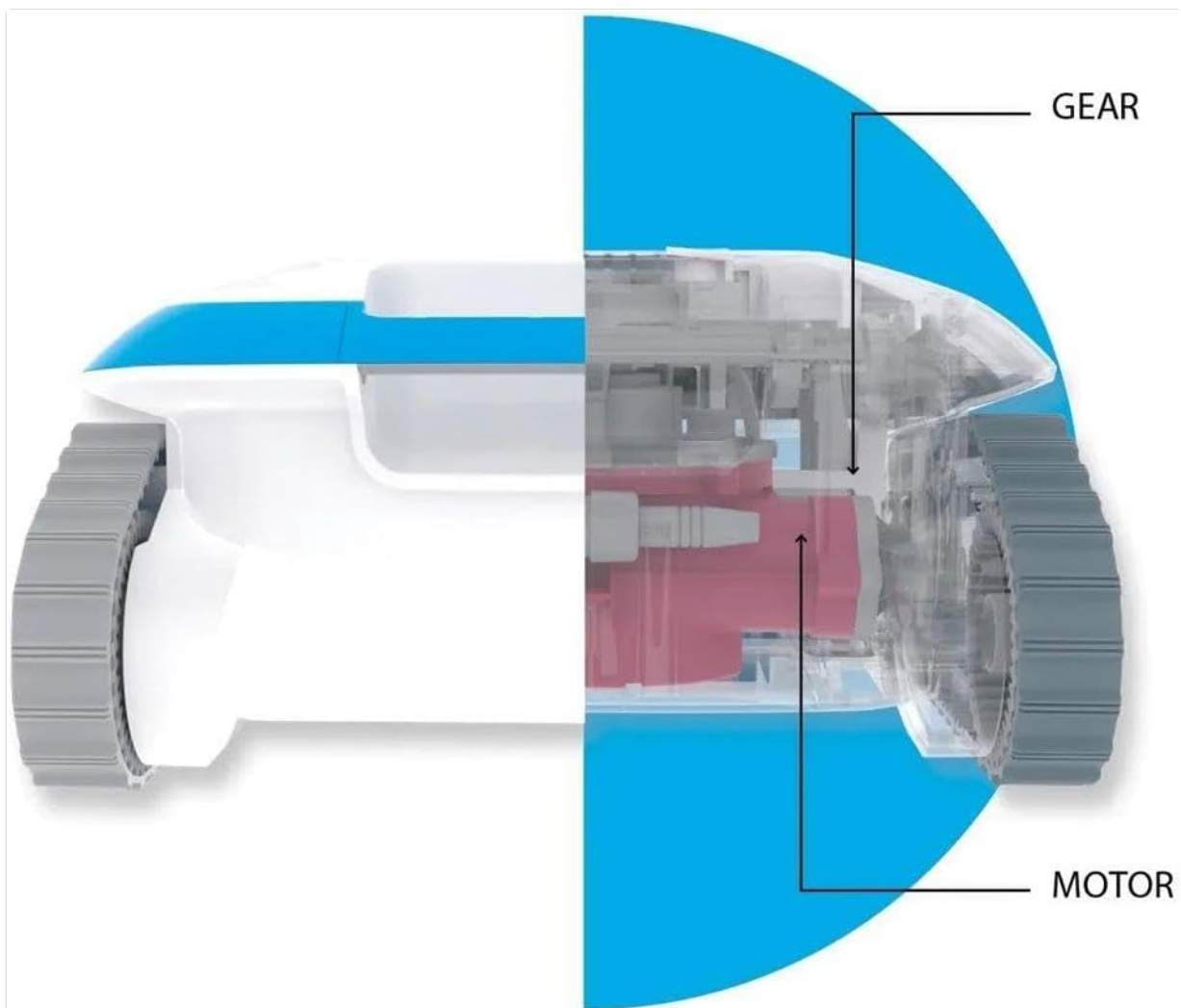
Image 3.3: Internal view of the cleaner, showing the gear and motor components responsible for its movement and cleaning action.
