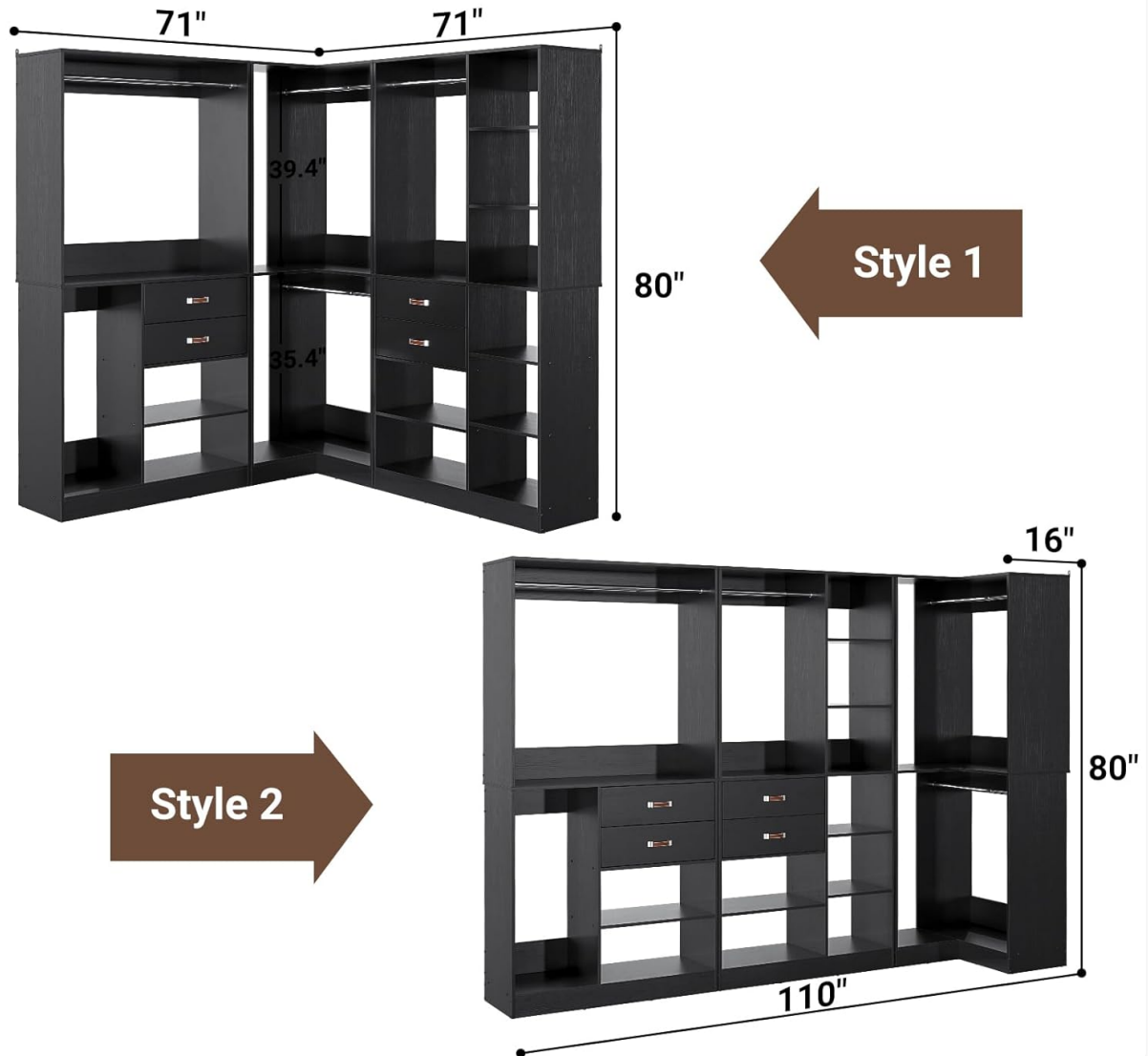
Image 4.2: Dimensional breakdown for Style 1 (standard L-shape) and Style 2 (extended configuration).
