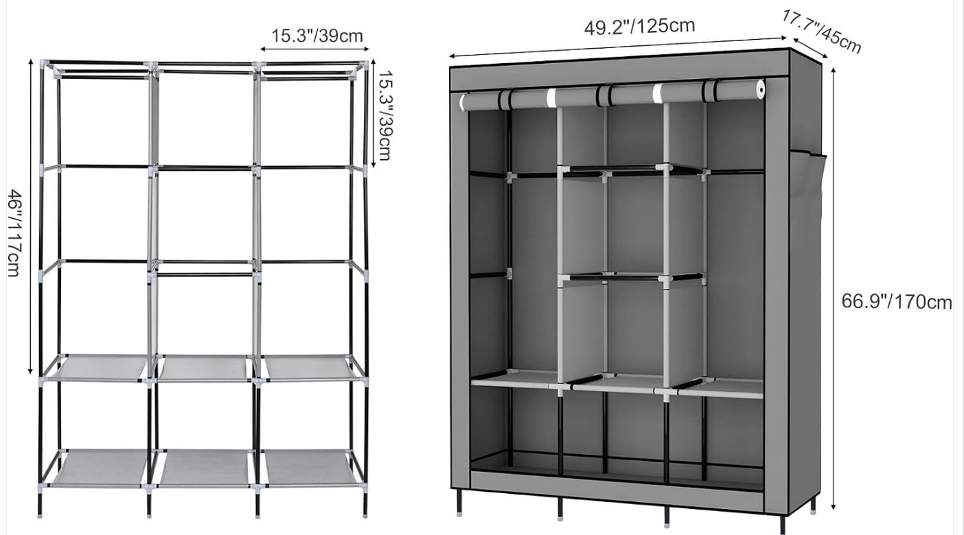
Image: Dimensions of the assembled SortWise Portable Closet frame and with cover.
