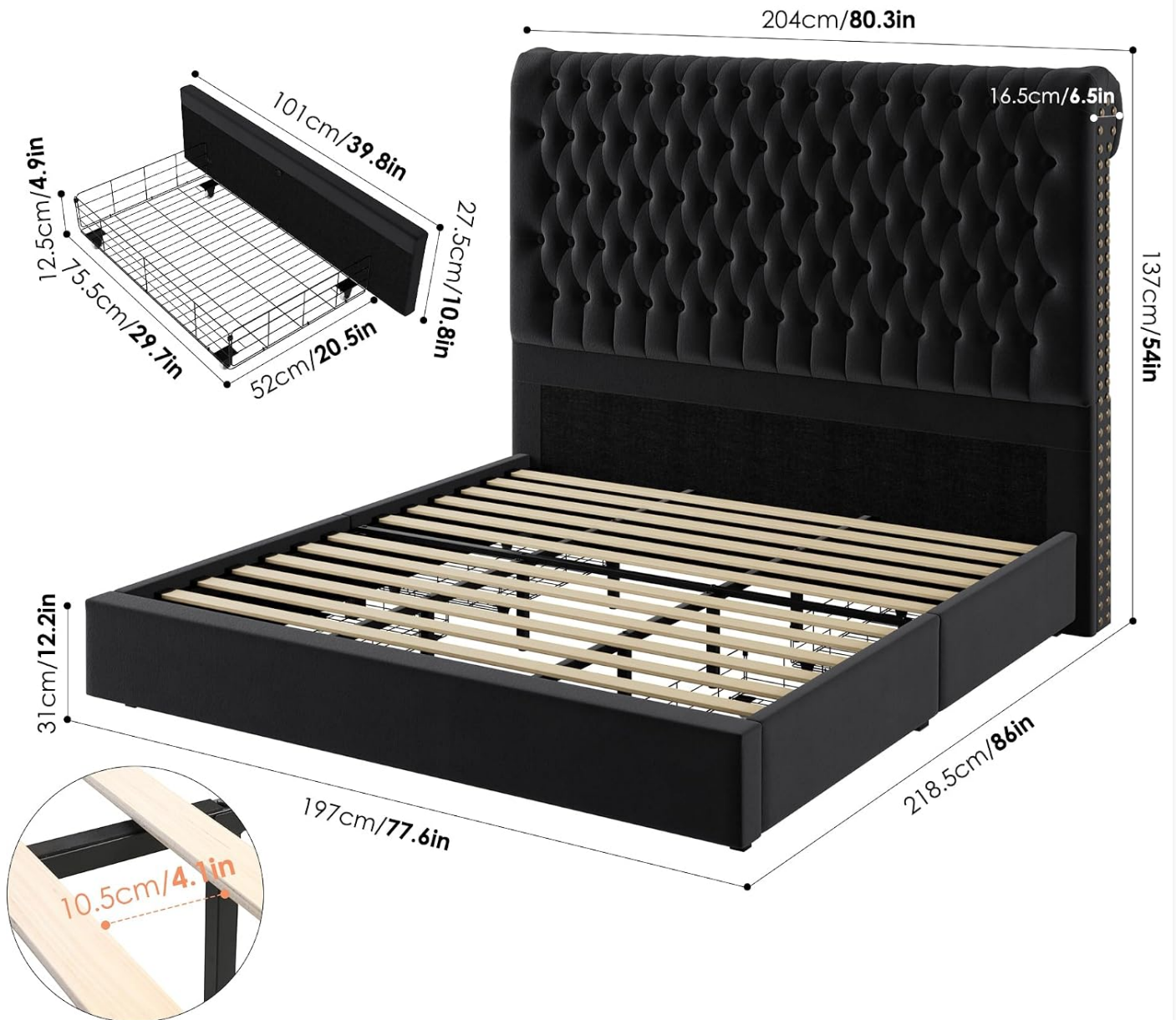
Image 8.1: Dimensional diagram of the Keyluv King Size Bed Frame, including headboard height, overall length, and width.
