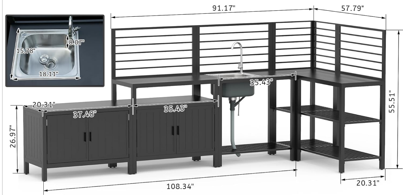
Figure 8.1: Overall dimensions of the 5-piece outdoor kitchen island.
