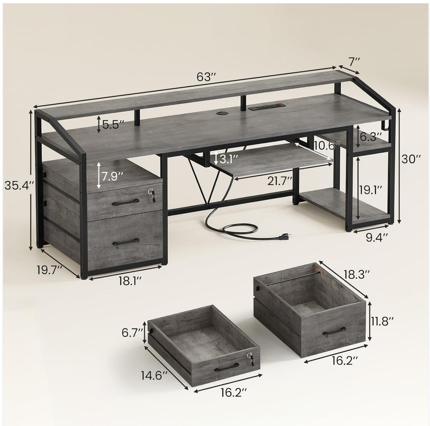
Figure 4.1: Desk Dimensions. This diagram illustrates the overall dimensions of the desk, including the 63-inch length, 19.7-inch depth, and 35.4-inch height, along with detailed measurements for the monitor stand, keyboard tray, and storage compartments.
