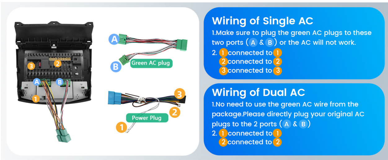
Image: AC wiring diagrams for single and dual AC systems.
