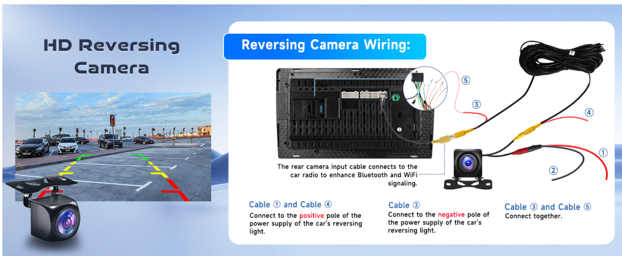
Image: HD Reversing Camera wiring diagram.
