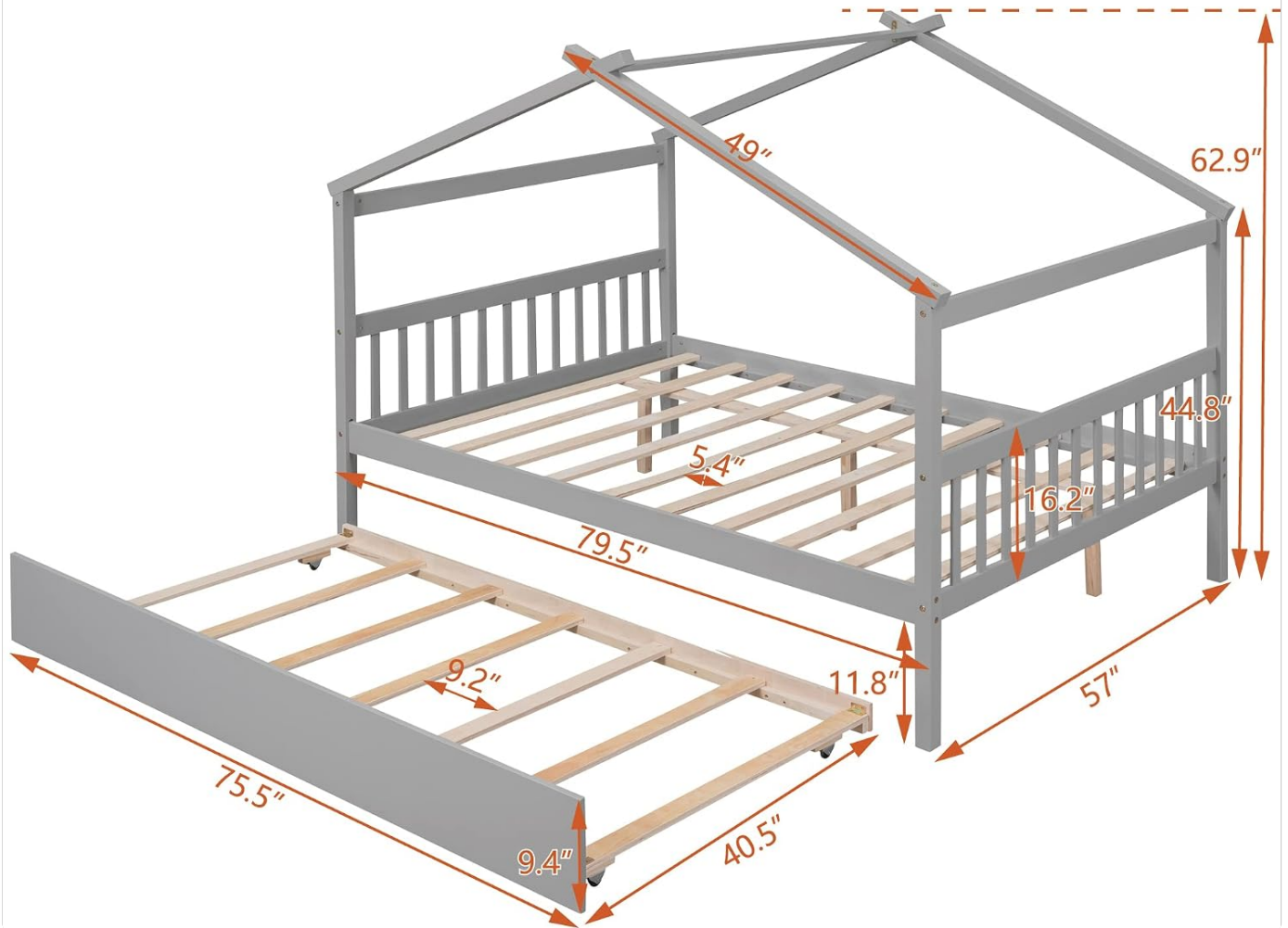
Image 1: Overall dimensions and structural overview of the bed.
