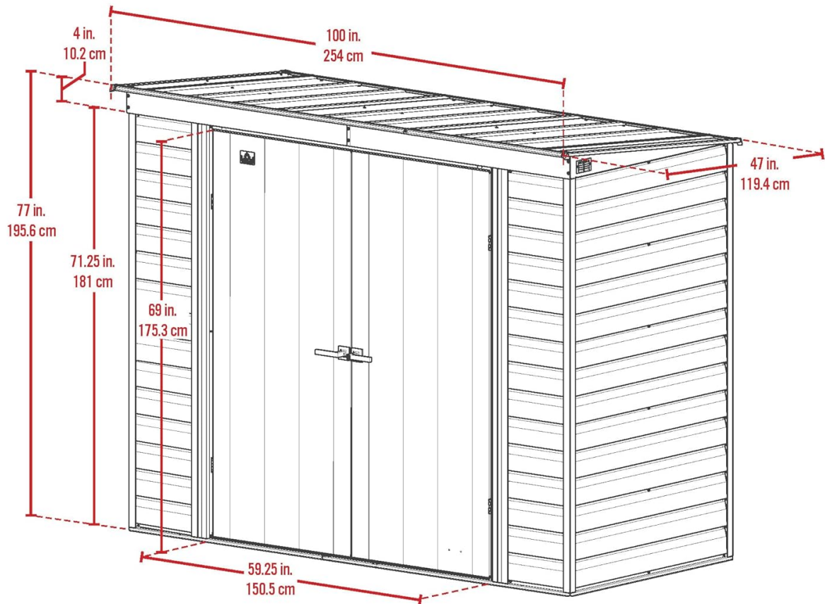
Image 4.1: Dimensional drawing of the shed, showing key measurements.
