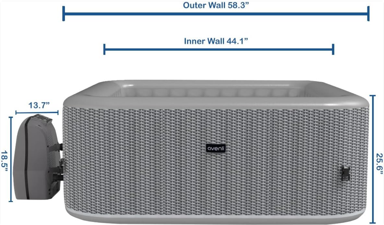
Figure 8.1: Key dimensions of the Avenli Inflatable Square Spa.
