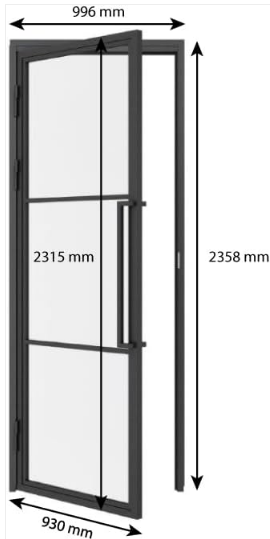
Figure 3: Door Dimensions
