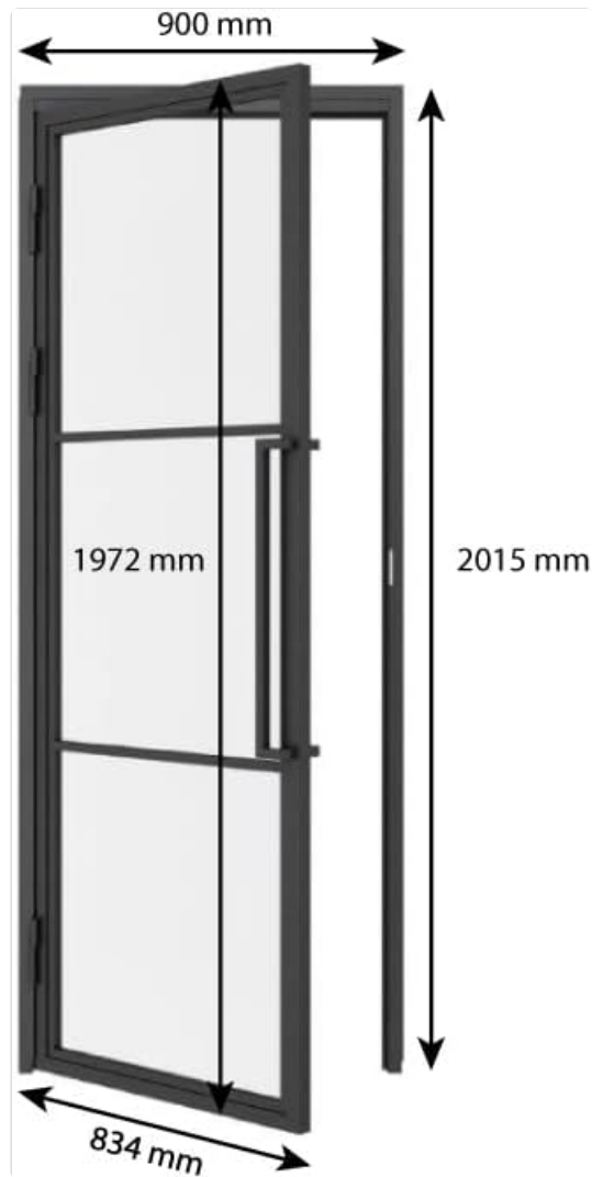
Image: Technical diagram illustrating the precise dimensions of the door and its components.
