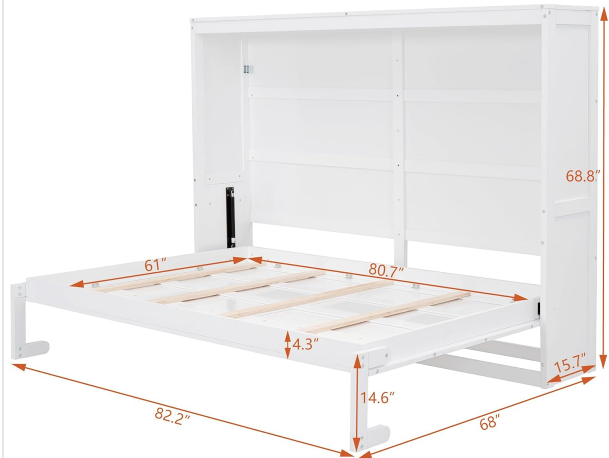
Figure 1: Dimensions of the Merax Queen Murphy Bed in open position. Overall length 82.2 inches, width 68 inches, height 68.8 inches.
