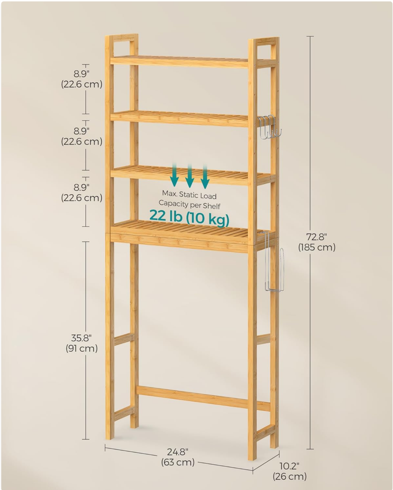
Image 6.1: Dimensional overview of the storage unit.
