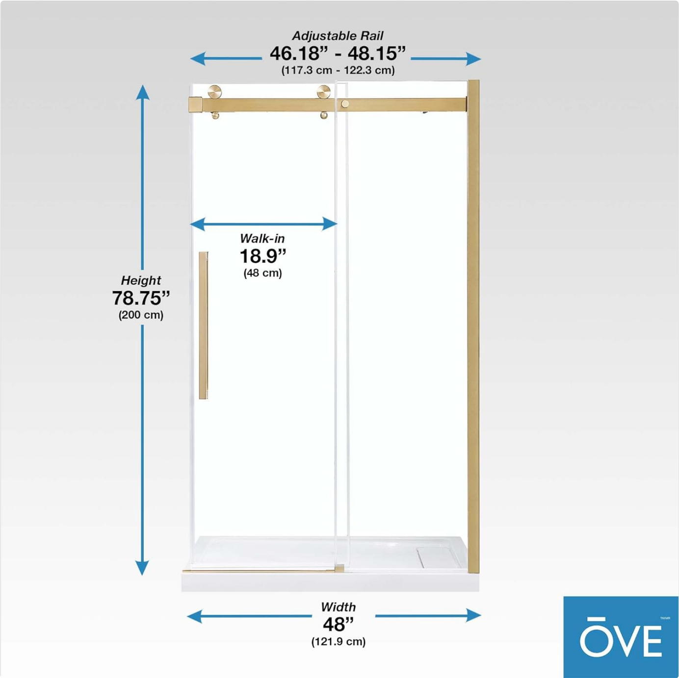
Image: Diagram illustrating the dimensions of the OVE Decors Bel shower door, showing an adjustable rail width of 46.18-48.15 inches, a height of 78.75 inches, and a walk-in width of 18.9 inches.
