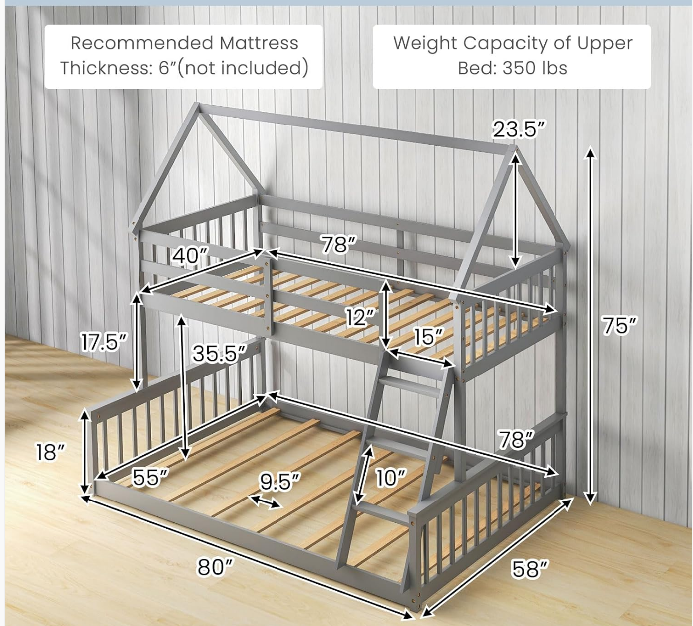
Figure 1: Product Dimensions. This diagram illustrates the overall length, width, and height of the bunk bed, along with specific measurements for the upper and lower bunks, ladder, and guardrails. The recommended mattress thickness is 6 inches, and the upper bed capacity is 350 lbs.
