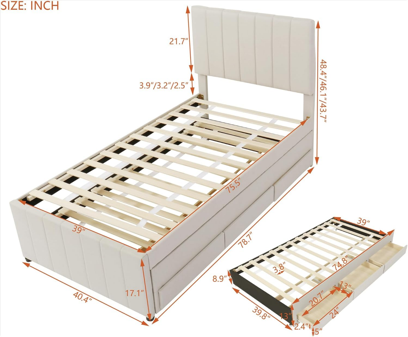
Image 8.1: Detailed dimensions of the Brabrety Twin Upholstered Platform Bed.
