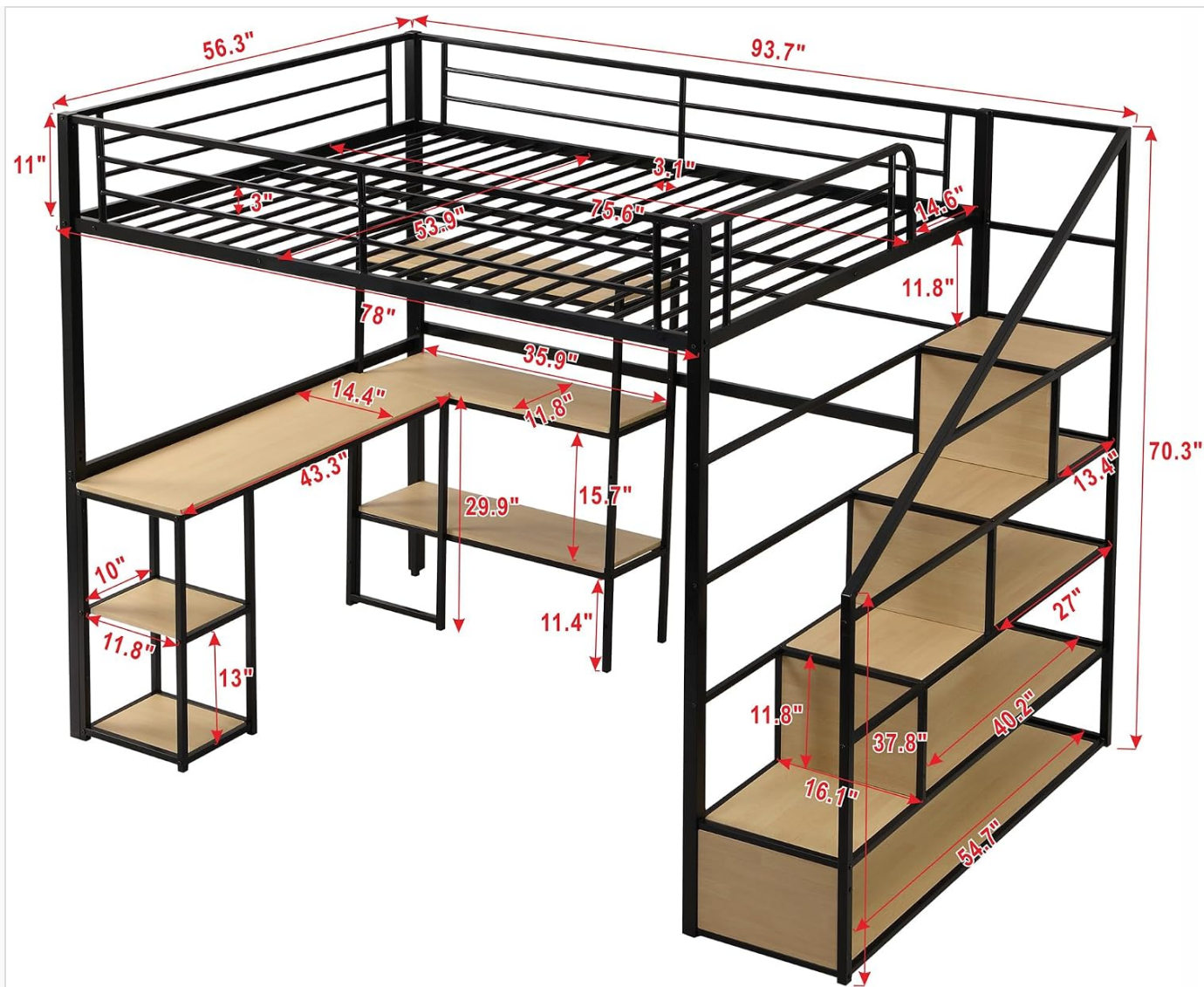
Image 8.1: Detailed diagram showing the dimensions of the KLMM Full Size Loft Bed.
