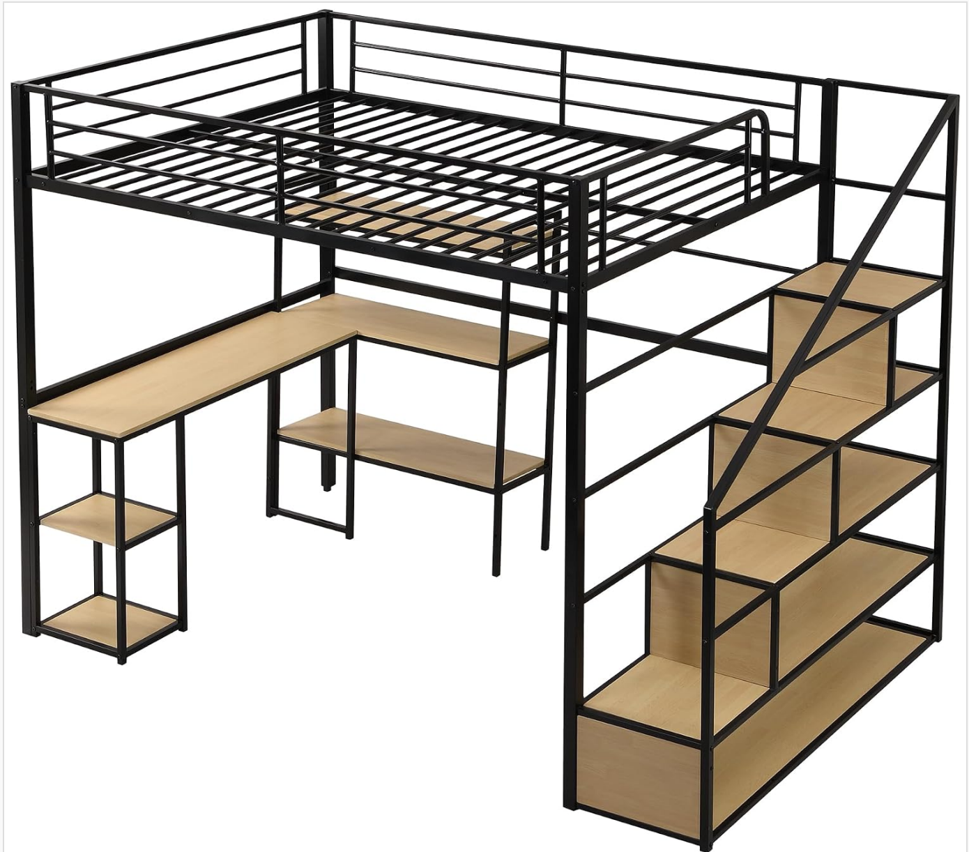
Image 3.1: Structural view of the loft bed, showing metal frame and MDF components.
