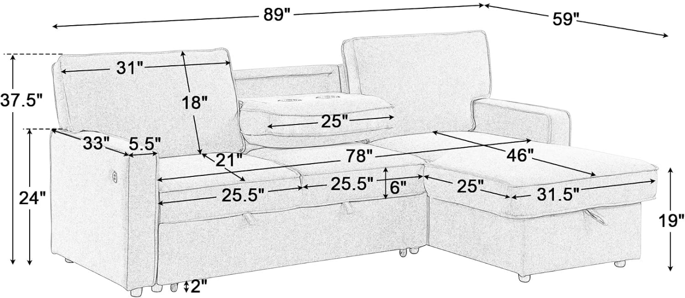
Image: Detailed diagram illustrating the dimensions of the sofa and its various components.
