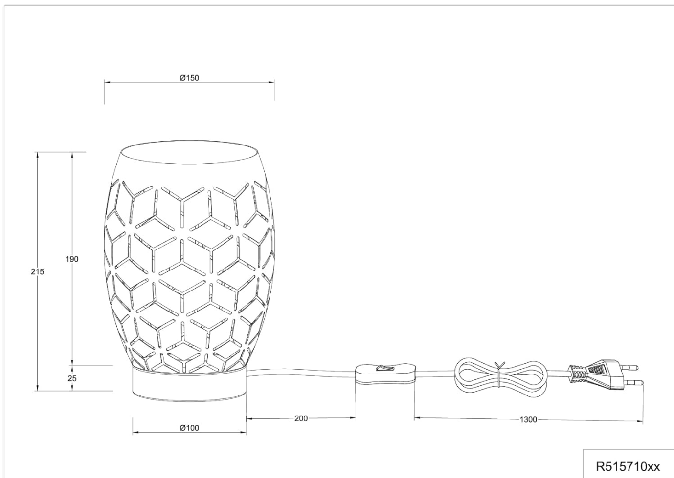
Figure 3: Technical drawing with product dimensions.
