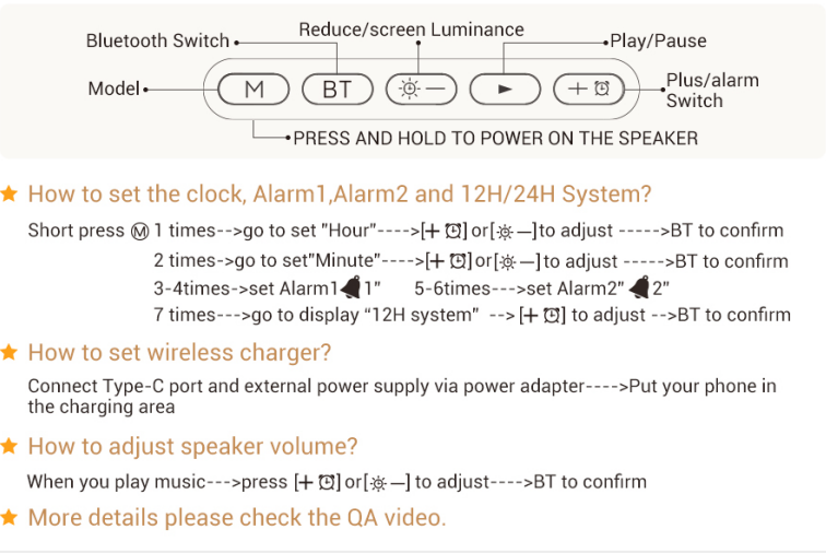
Figure 4.1: Control panel layout and detailed instructions for setting clock and alarms.
