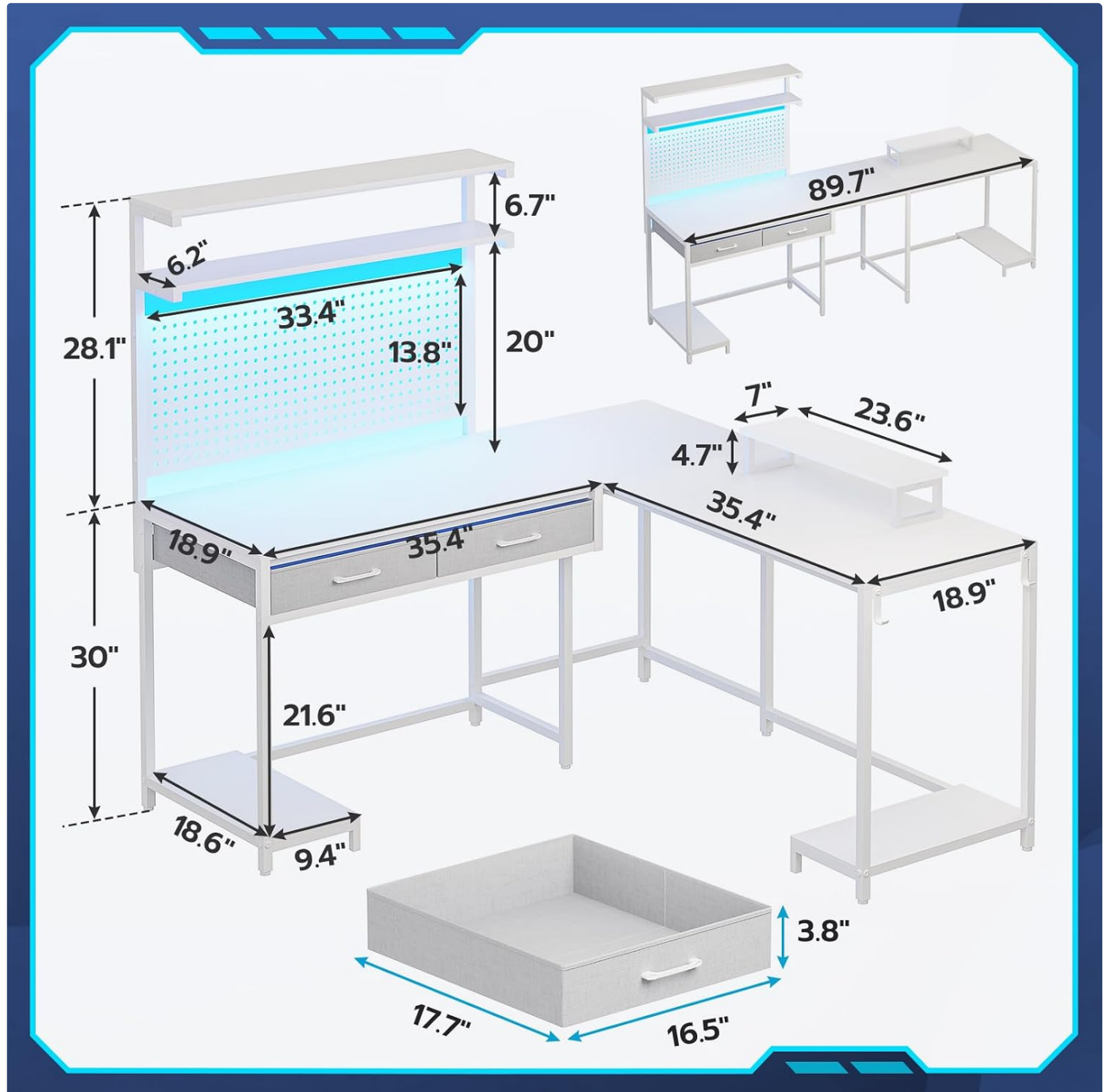
Figure 4.1: Dimensional diagram of the desk, illustrating key measurements for assembly and placement.
