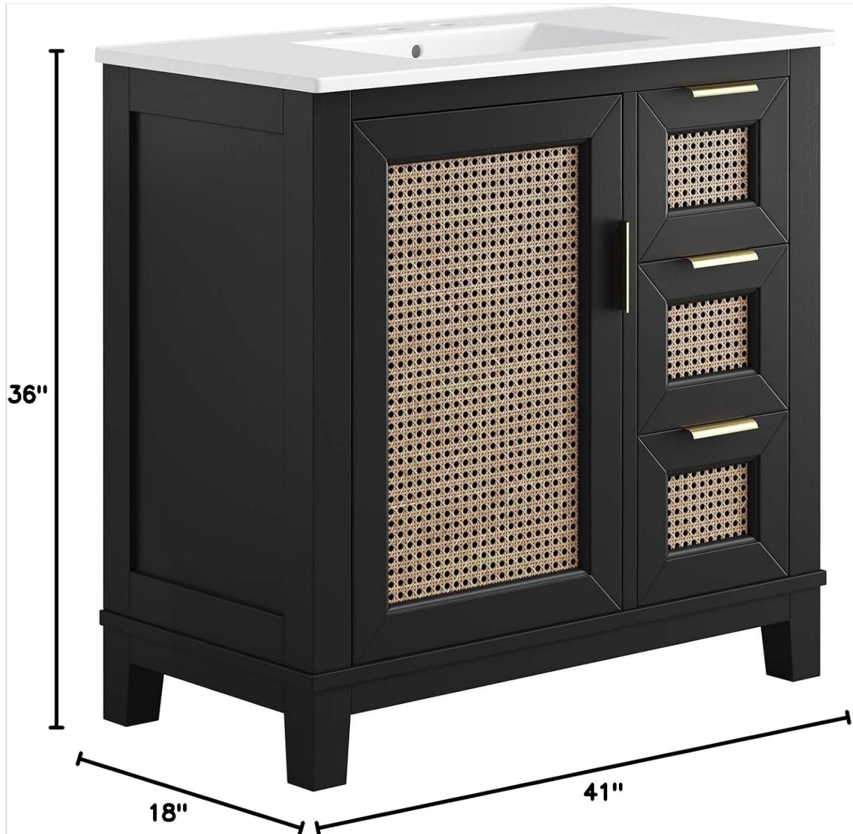
Figure 5: Dimensional diagram of the Modway Dixie 36-inch Bathroom Vanity Cabinet.
