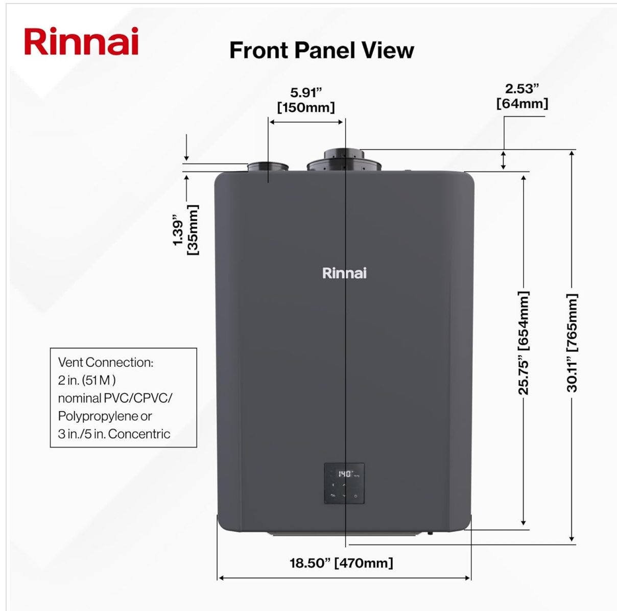
Figure 5.1: Front Panel View with Dimensions and Venting Information
