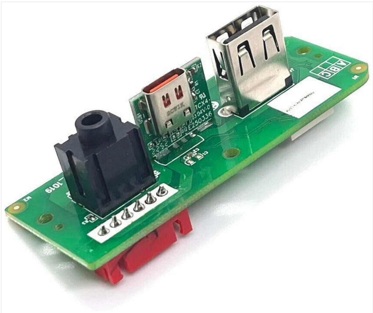
Figure 3: Detailed view of the board's ports and connectors, crucial for installation.
