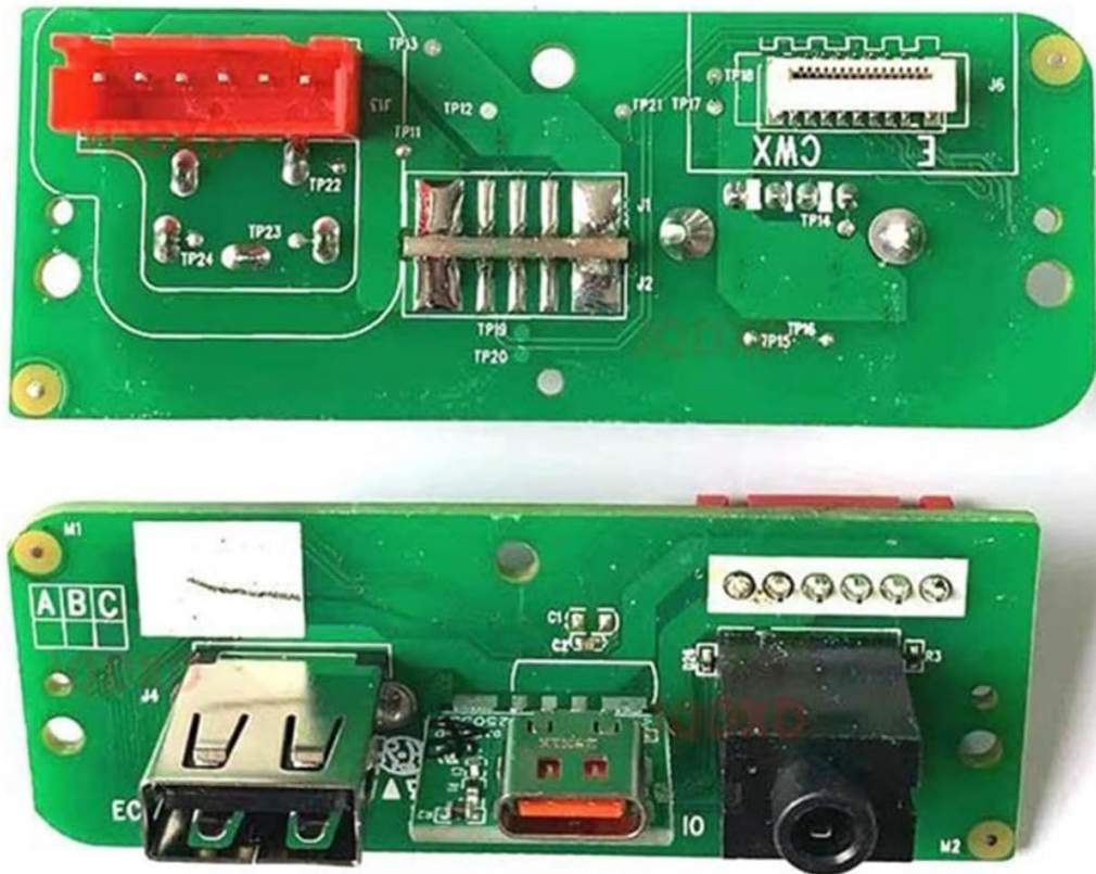
Figure 1: ZEZEUFU Charging Port Board, highlighting compatibility with JBL Xtreme 3 GG.
