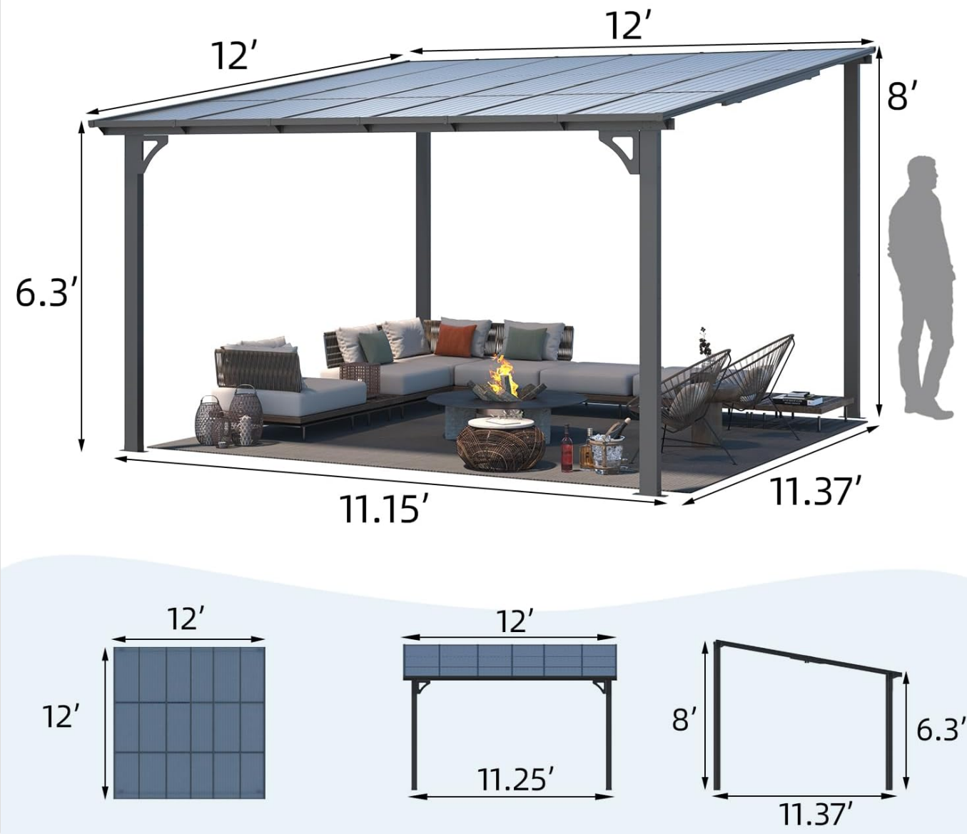
Image: Detailed dimensions of the 12' x 12' hardtop gazebo.
