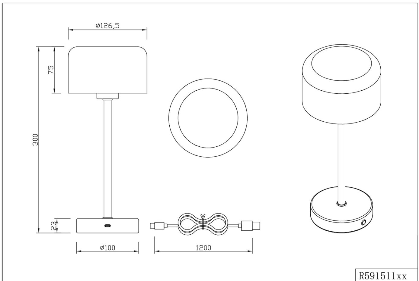
Image: Diagram showing the lamp's dimensions and the included USB-C charging cable.
