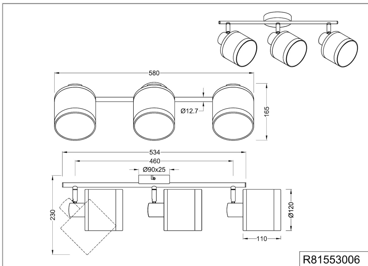
Figure 1: Technical drawing showing dimensions and mounting points for the R81553006 spotlight bar. Dimensions are in millimeters.
