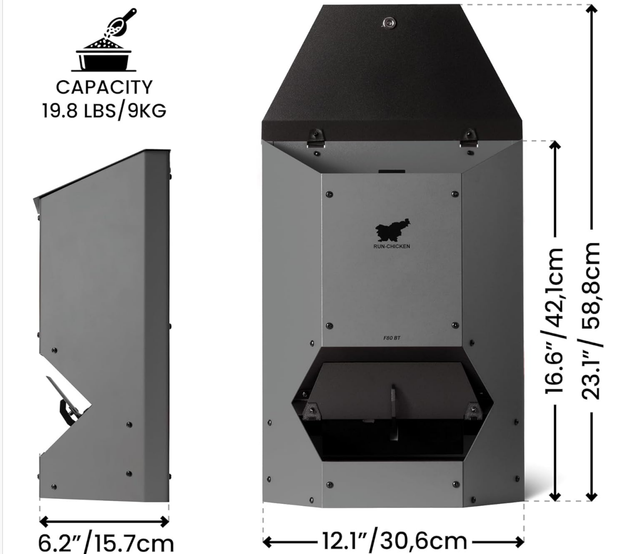
Image 7.1: Detailed dimensions and capacity of the F80 Feeder.
