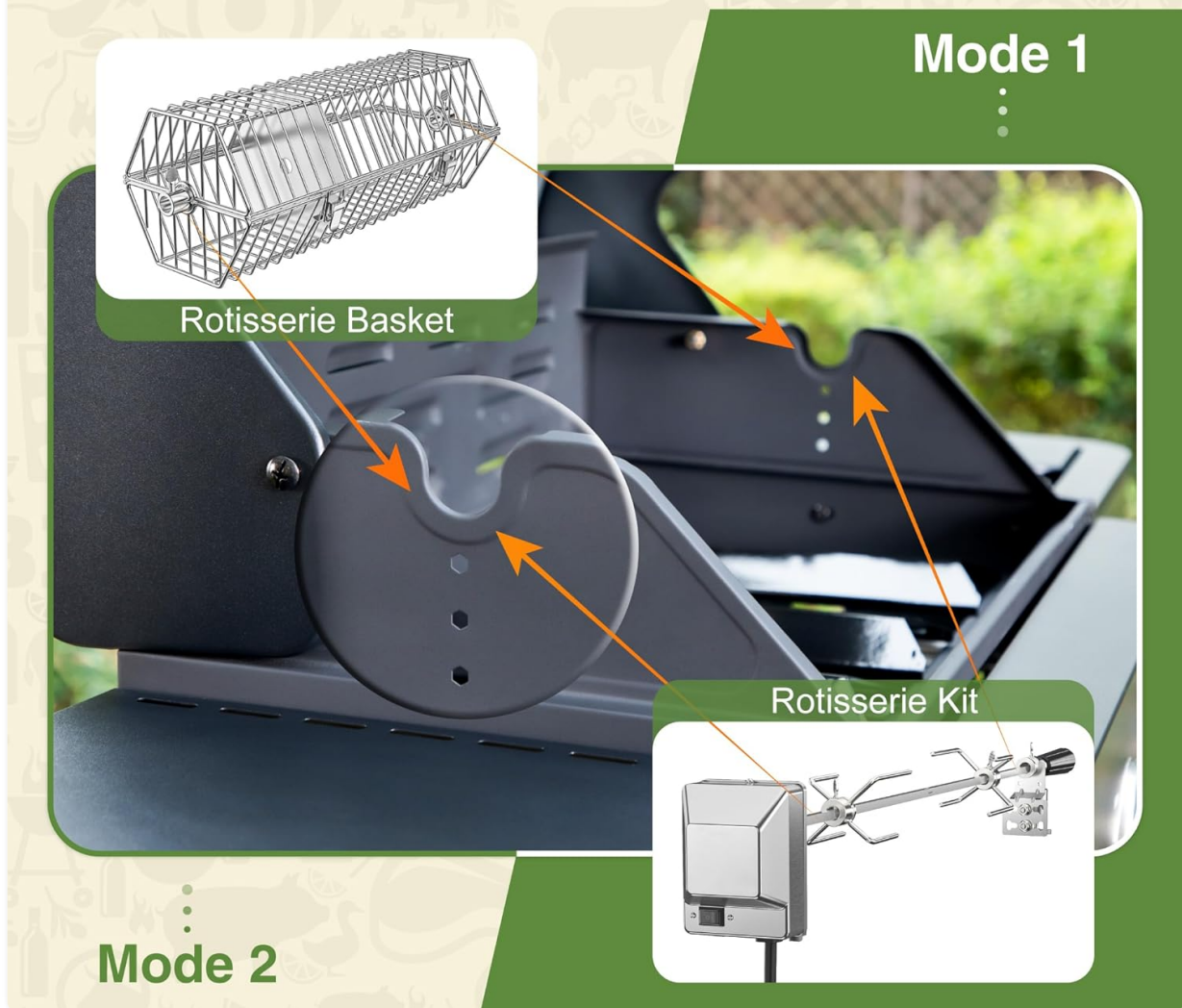
Image 6.5: Designated slots for installing an optional rotisserie kit or basket.
