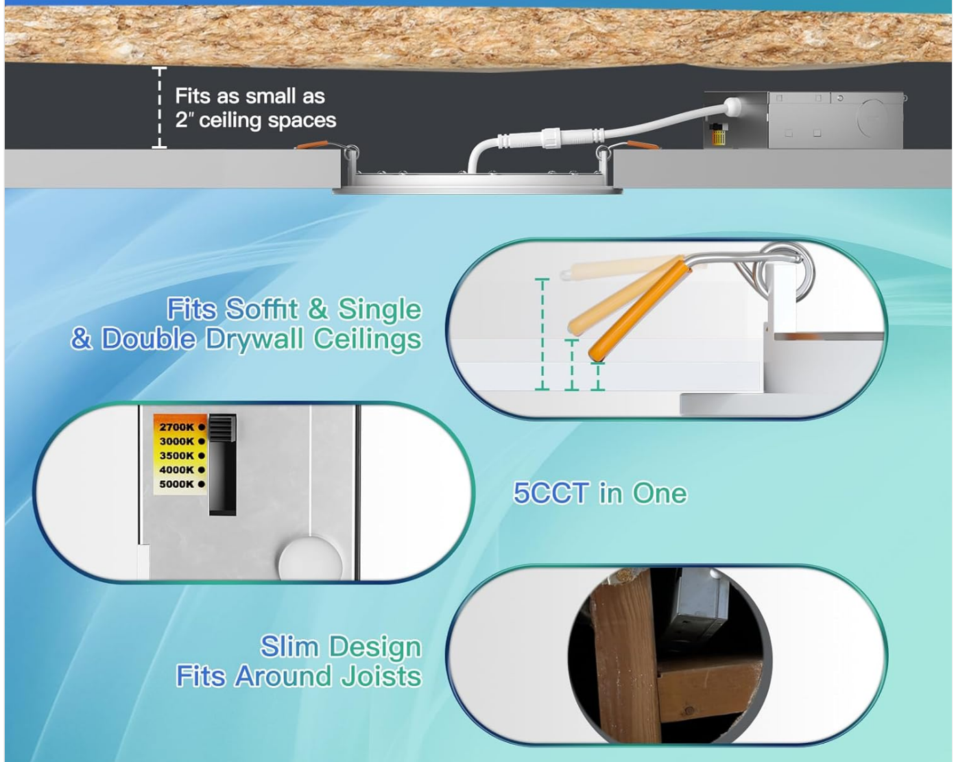
Figure 3: Installation Flexibility in Various Ceiling Types.
