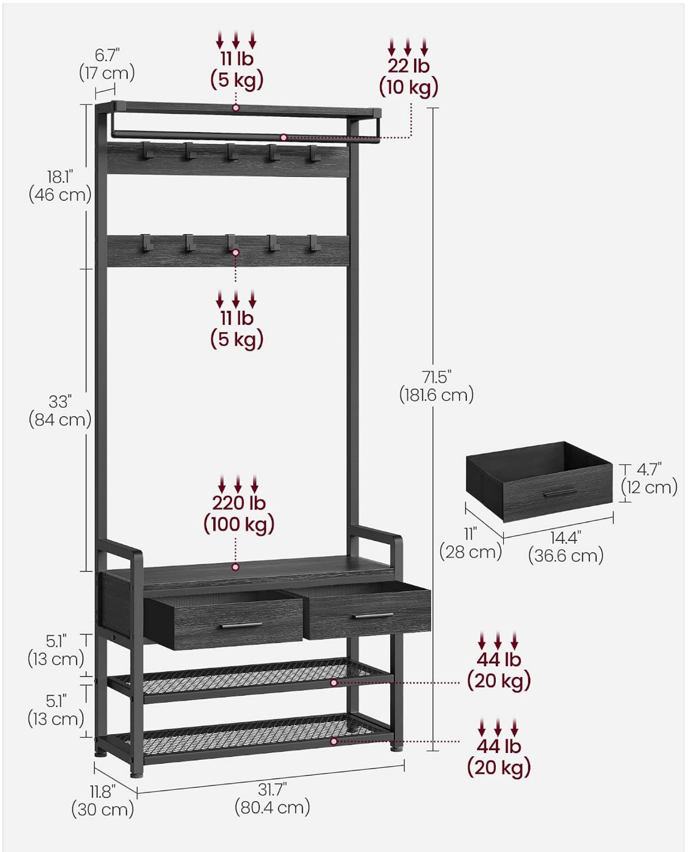
Image: Technical diagram displaying the overall dimensions and individual weight capacities for various parts of the hall tree.
