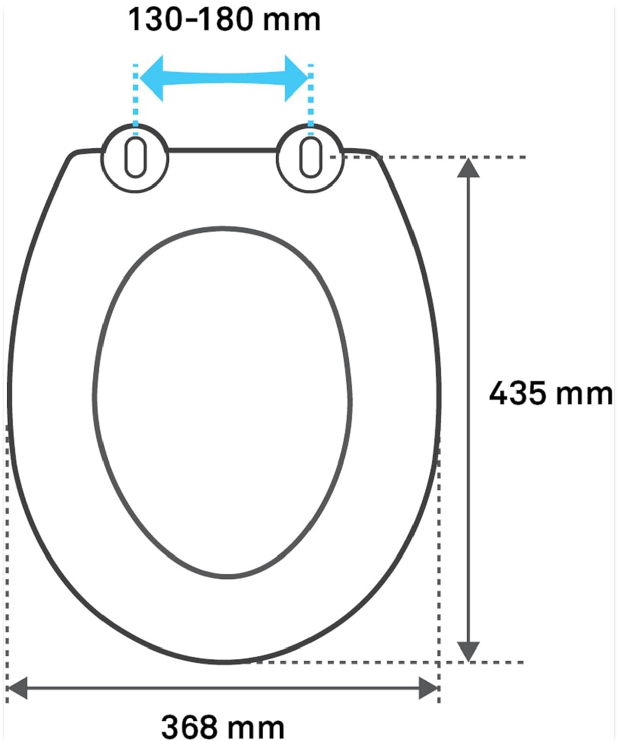
Figure 4: A technical diagram illustrating the key dimensions of the toilet seat: length 435 mm, width 368 mm, and adjustable hinge spacing between 130-180 mm.
