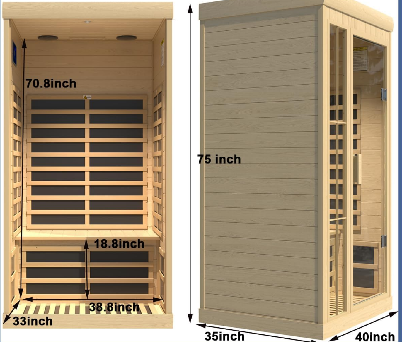
Image: Detailed dimensions of the sauna, including height, width, and depth.
