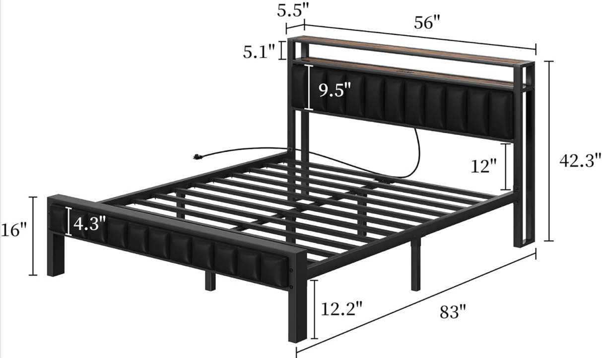
Image: Detailed dimensions of the LUXOAK Full Size Bed Frame.
