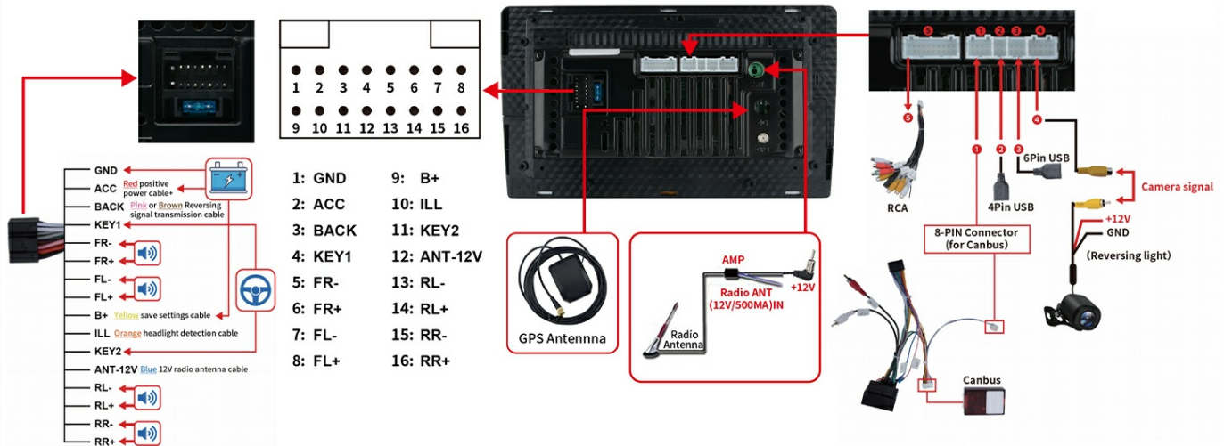
Image: A comprehensive wiring diagram illustrating how to connect the various cables from the head unit to the vehicle's electrical system and peripherals.
