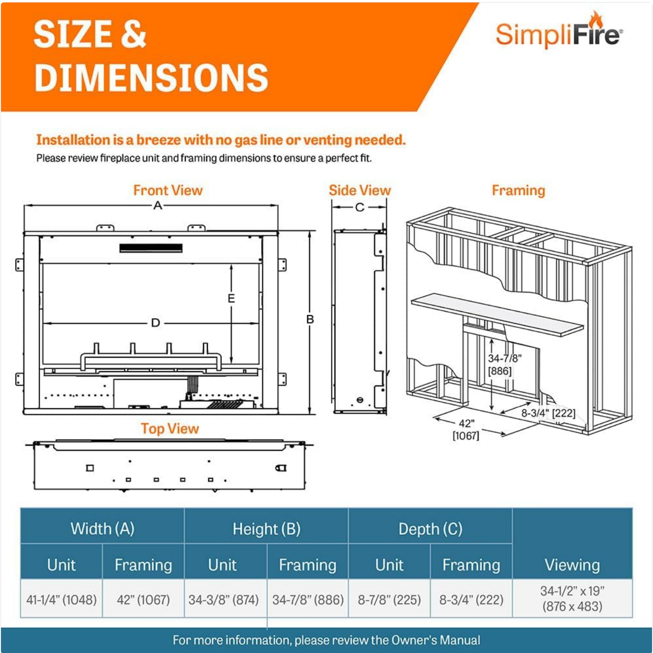
Figure 3.1: Detailed size and dimensions for the SimpliFire Inception Electric Fireplace, including front, side, and top views, and framing requirements.
