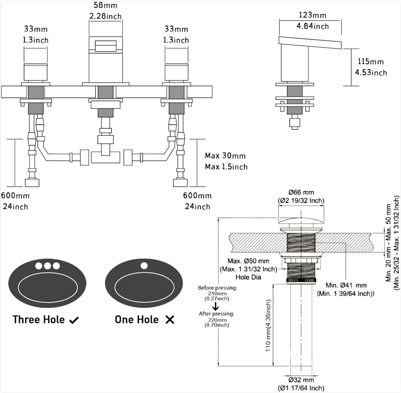
Figure 1: Overview of all included components for the AVSIILE LED Waterfall Bathroom Faucet, including the main spout, handles, drain, and installation hardware.
